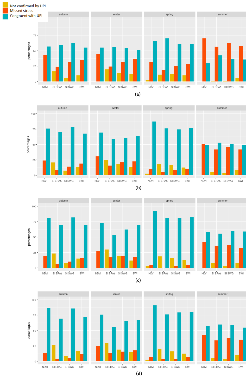
Figure 10. Probability of drought detection based on UPI and lagged UPI during the period between 2007 and 2019. (a) Stress identification basing on UPI. (b) Stress identification basing on a UPI 2 decade moving average. (c) Stress identification basing on UPI 3 decade moving average. (d) Stress identification basing on UPI 4 decade moving average.
